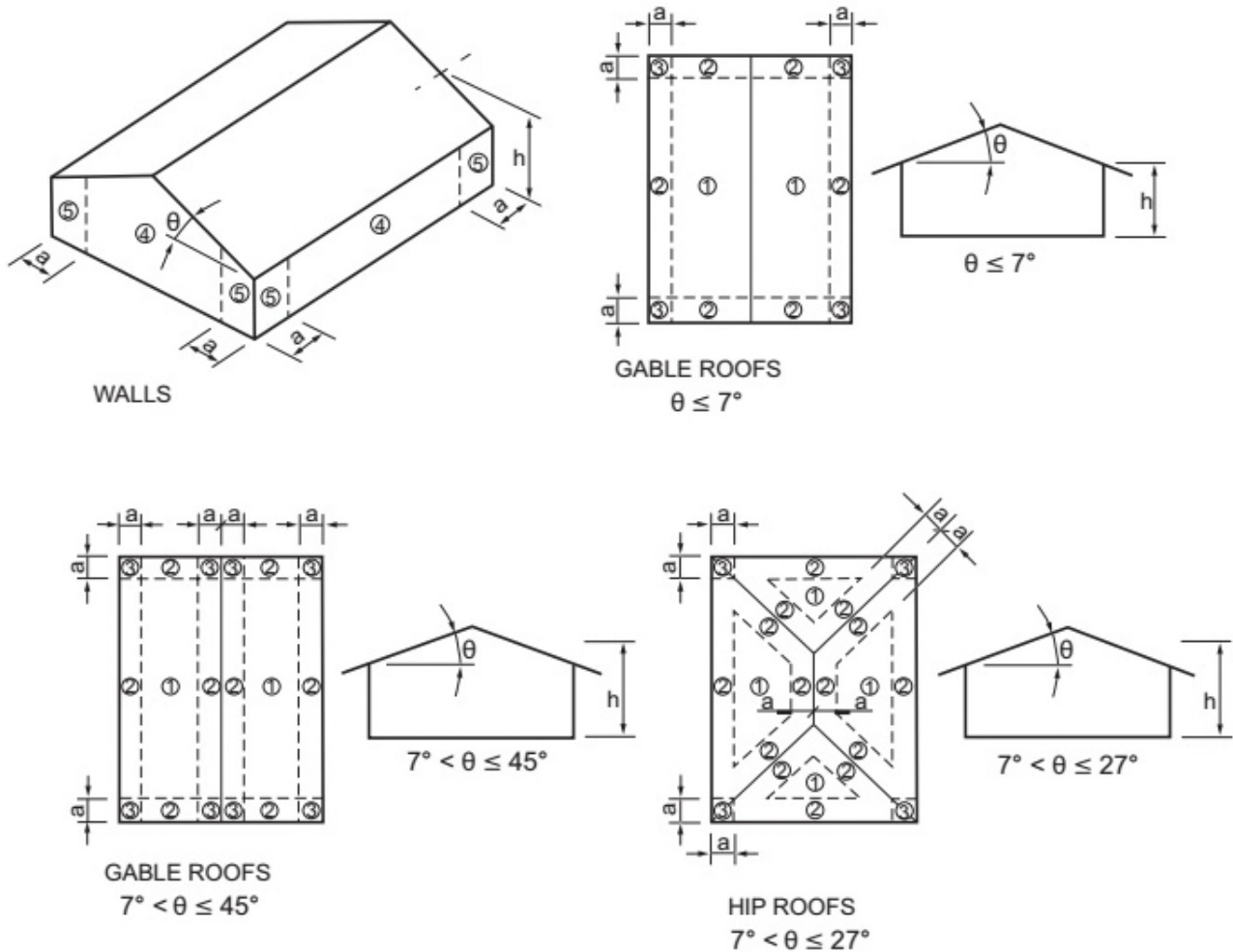
FIGURE R301.2(8) COMPONENT AND CLADDING PRESSURE ZONES
