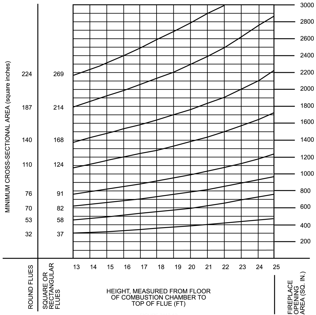
FIGURE 2113.12 FLUE SIZES FOR MASONRY CHIMNEYS
