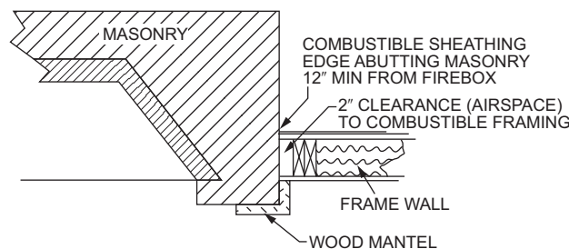
FIGURE 2111.12 ILLUSTRATION OF EXCEPTION TO FIREPLACE CLEARANCE PROVISION
