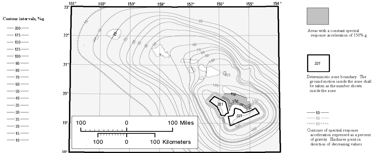
0.2 Second Spectral Response Acceleration (5% of Critical Damping)
