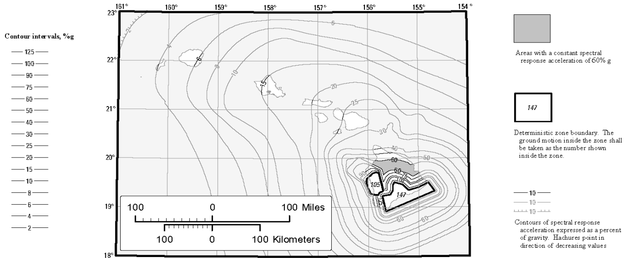
1.0 Second Spectral Response Acceleration (5% of Critical Damping)
