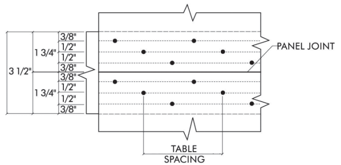
4" NOMINAL—THREE LINES
