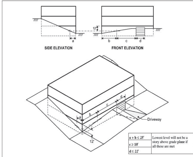
FIGURE 202S STORY ABOVE GRADE PLANE
