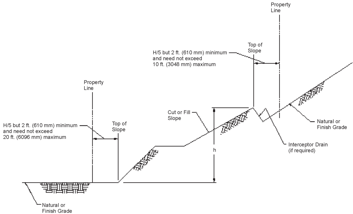
FIGURE J108.1 DRAINAGE DIMENSIONS
